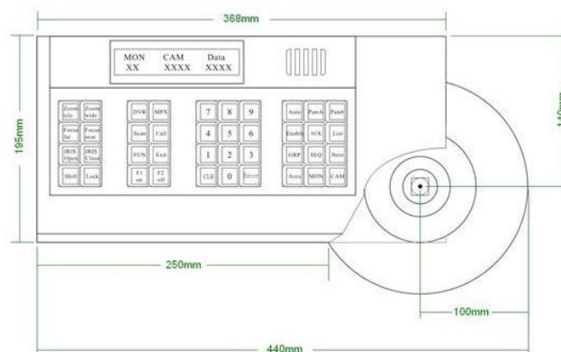
Mechanical Drawing
